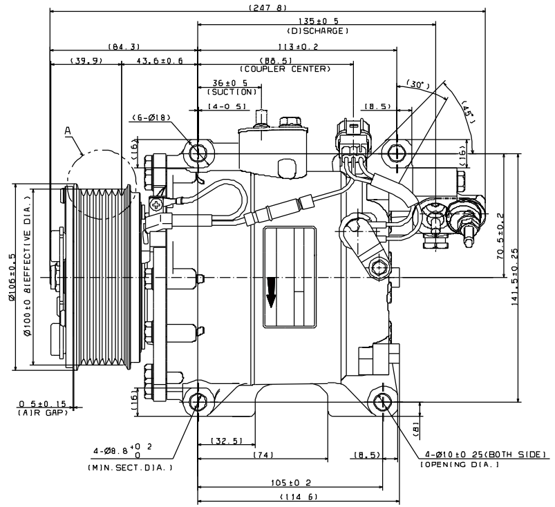
SECT SS
