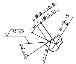
DETAIL E (5:1)
