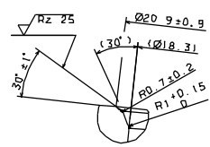
DETAIL F (5:1)
