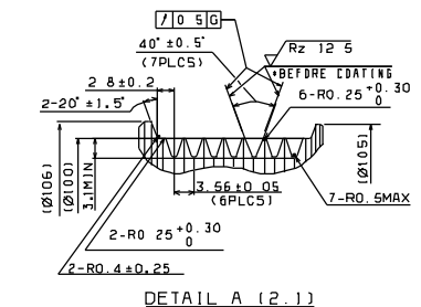
DETAIL A (2:1)
